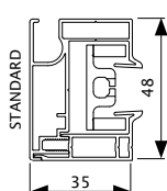
Coupling side channel (K)
