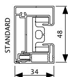
Coupling side channel (K)
