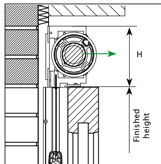
Installation method 5
