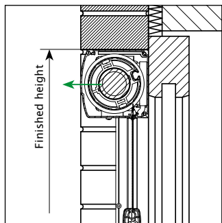
Installation method 1
