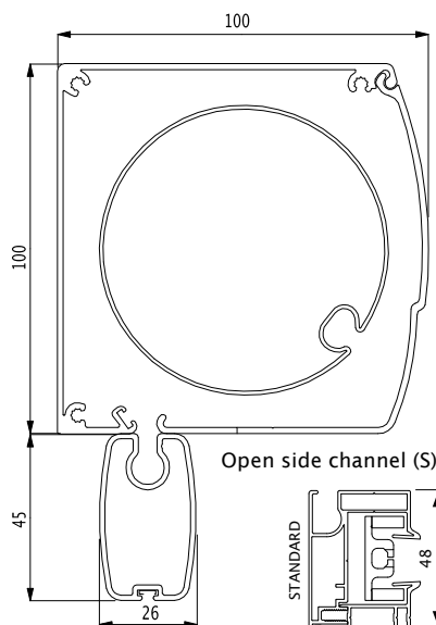
Closed side channel (G)
