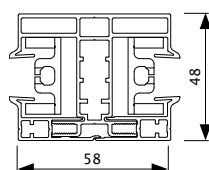
Coupling side channel (K)
