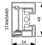
Side channel (S)
