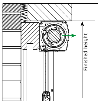
Installation method 6
