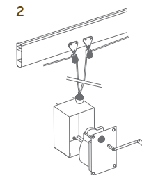
CRANK CONTROL WITH BAR MOUNTED ON THE WALL
